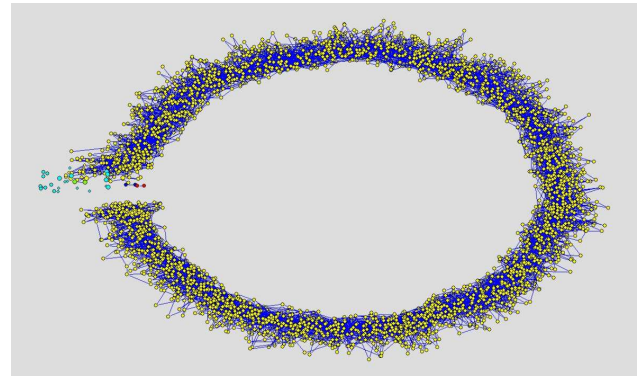
Fig. 2. Circular FR plot of partitions of CSC under T_1 in the interval T_0=0 to T=644 . The picture shows one giant, connected lineage, and several small, isolated components (on the left).
