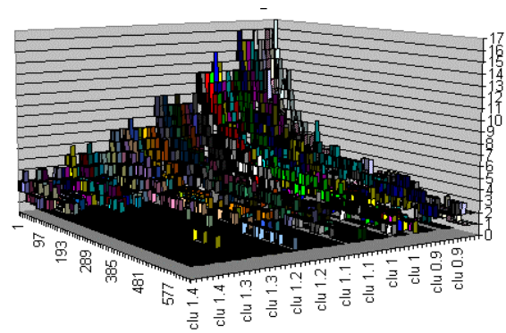
Fig. 3. Clusters against time. Convergence to (typically) one PSC cluster under T_1 for d_{cluster} \geq 1 . The Figure summarizes 60 runs, 10 for 6 random seeds each, from d_{cluster} = 0.9 to 1.4. Time goes left to right, the clustering constant increases right to left. Vertical axis shows number of clusters.
